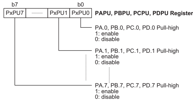
Pull-High Resistor Register – PAPU, PBP, PCPU, PDP
