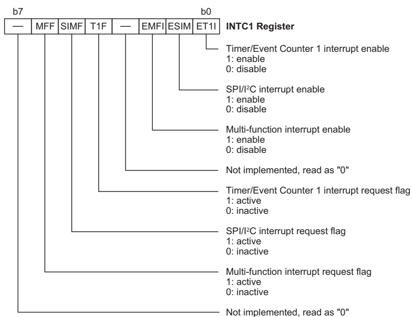
Interrupt Control Register – INTC1
