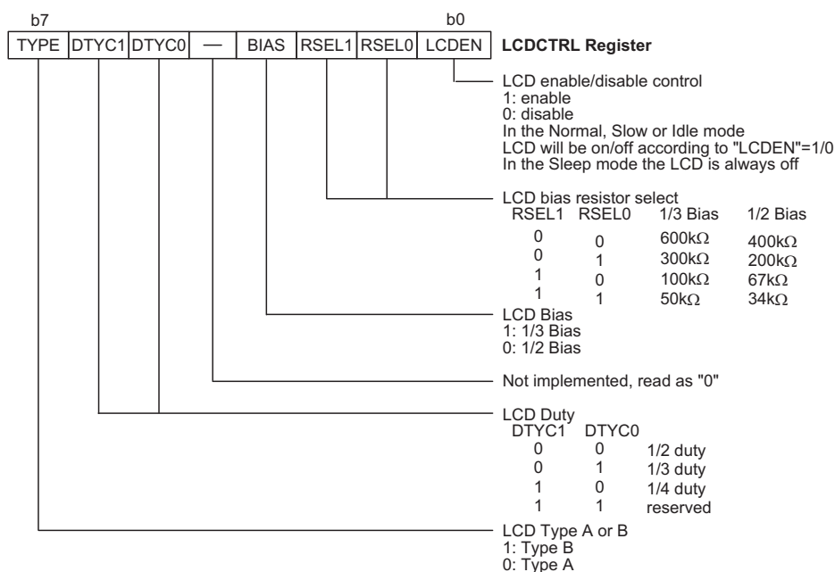
LCD Control Register – LCDCTRL - HT56R67
