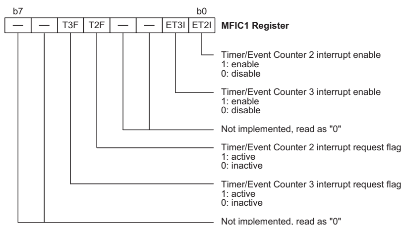
Interrupt Control Register – MFIC1
