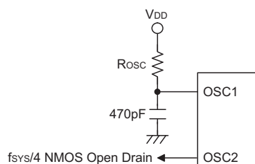
RC Oscillator
