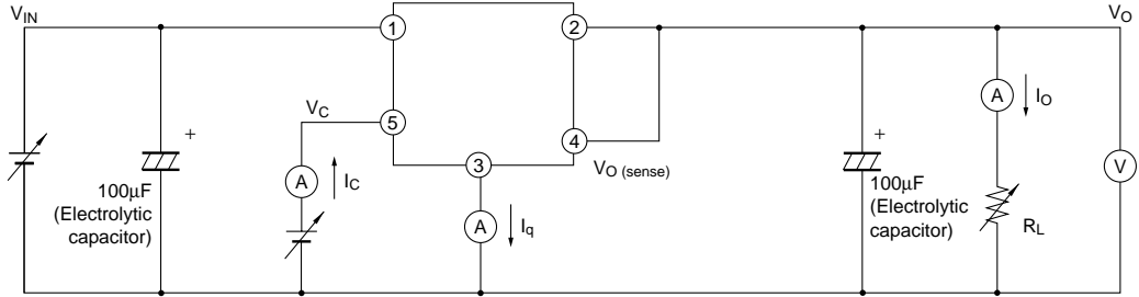
Fig.1 Standard Test Circuit
