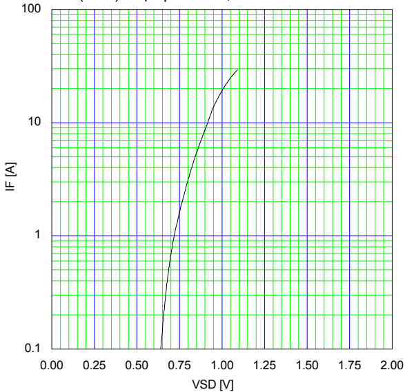
Typical Forward Characteristics of Reverse Diode I_F=f(V_{SD}):80\ \mu s\ pulse\ test, T_{ch}=25\text{ }^\circ\text{C}
