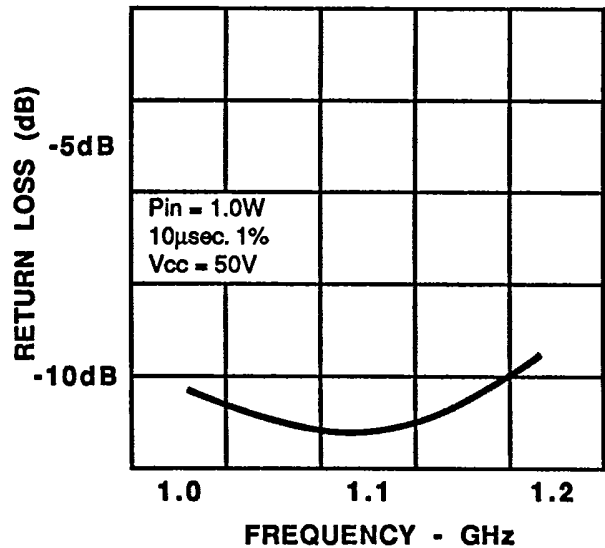
WIDEBAND CIRCUITRY INPUT RETURN LOSS (TYPICAL)
