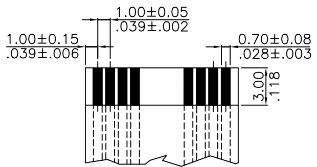
Recommended FFC/FPC Pattern Thickness 0.3mm (.012")
