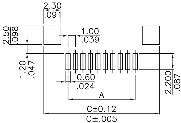
Recommended P.C.Board Pattern
