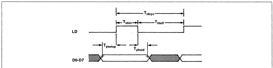
Parallel Interface Timing Waveforms
