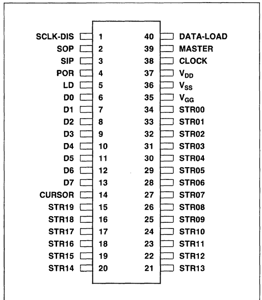
10939 Pin Configurations
