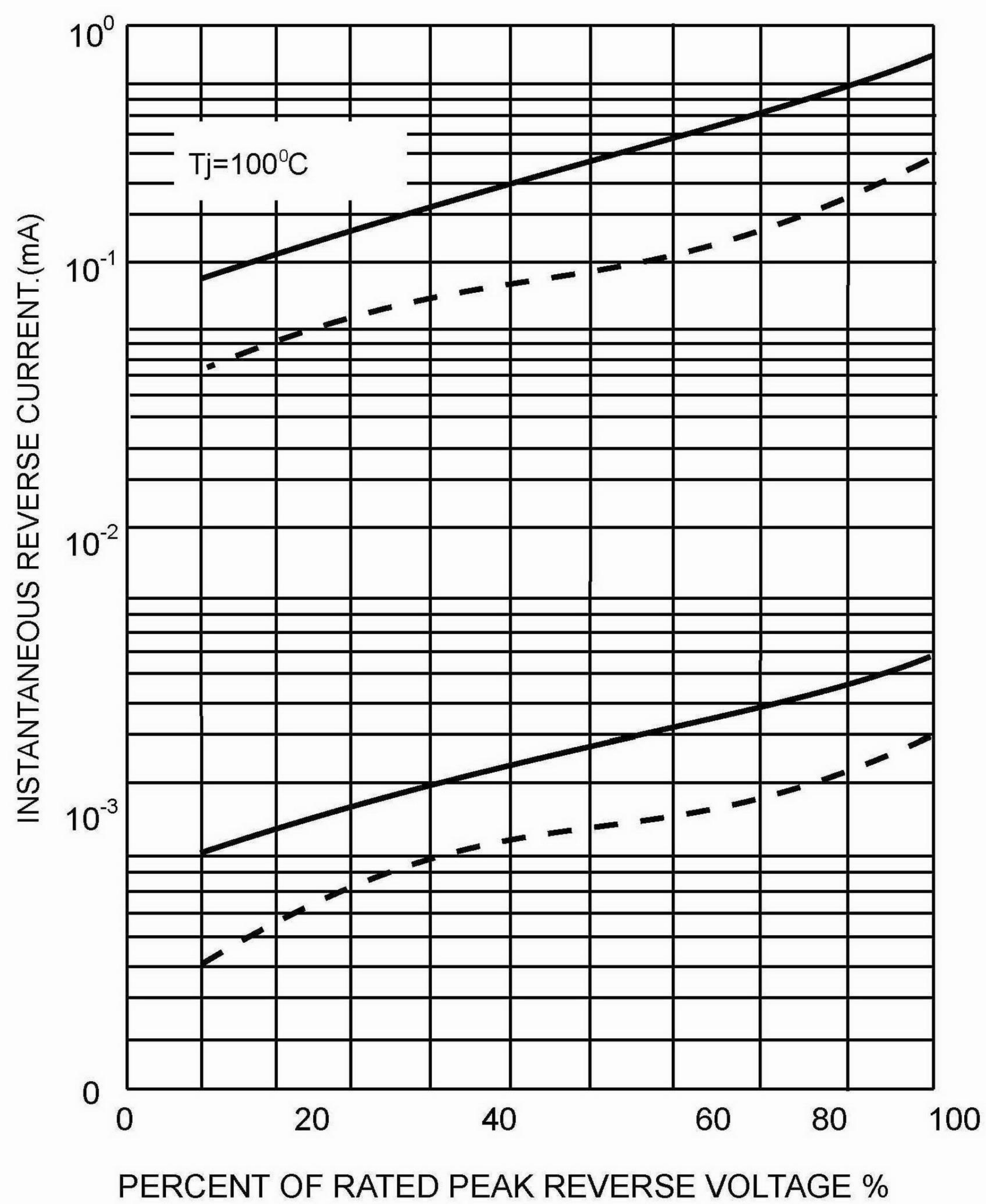
FIG.3-TYPICAL REVERSE CHARACTERISTIC
