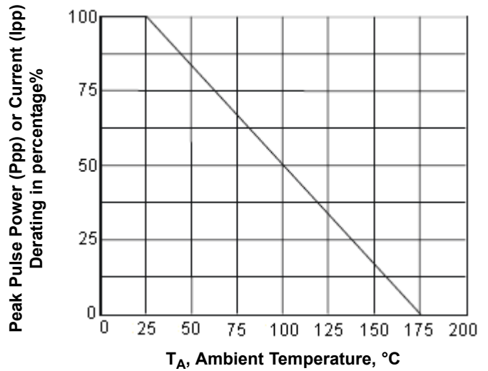
Fig. 2-Pulse Derating Curve
