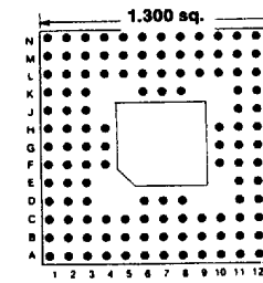
Footprint 13006
