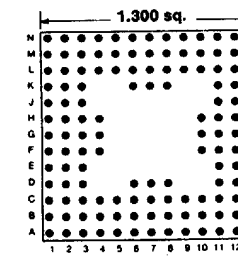
Footprint 13007
