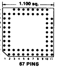
Footprint 11035
