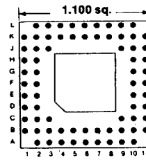
72 PINS Footprint 11026
