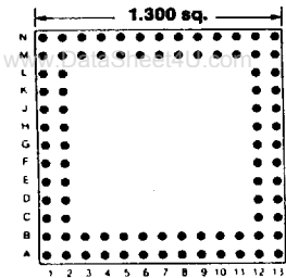
Footprint 13029
