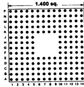
180 PINS Footprint 14003
