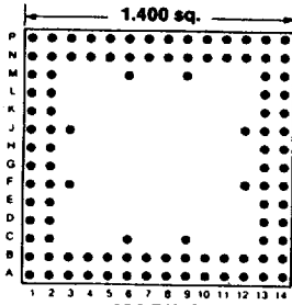
104 PINS Footprint 14018
