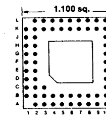
69 PINS Footprint 11030
