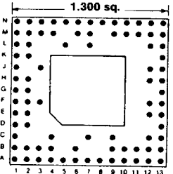
88 PINS Footprint 13049
