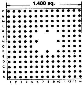
179 PINS Footprint 14005
