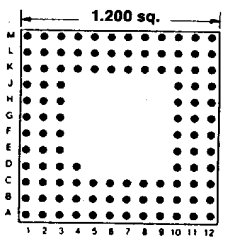
Footprint 12003
