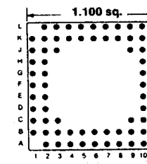
72 PINS Footprint 11025
