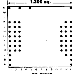
Footprint 13037
