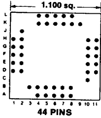
Footprint 11042
