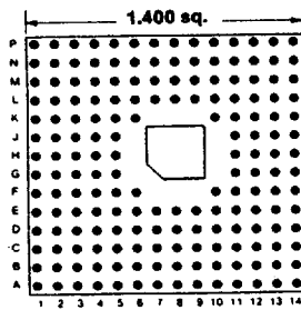
175 PINS Footprint 14004
