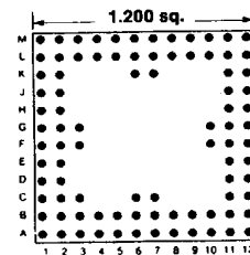
Footprint 12007
