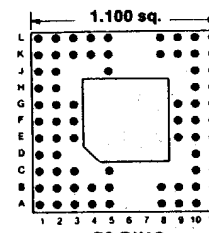
73 PINS Footprint 11019
