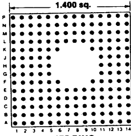
175 PINS Footprint 14006
