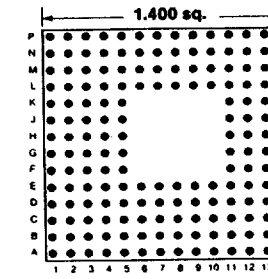
171 PINS Footprint 14008
