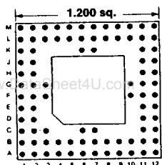
Footprint 12006
