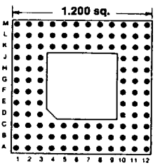
Footprint 12004
