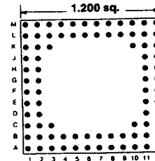
Footprint 12013
