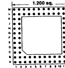
Footprint 12014
