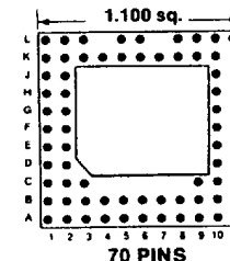
70 PINS Footprint 11028
