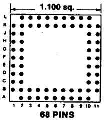
Footprint 11033
