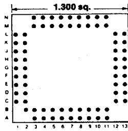
Footprint 13035
