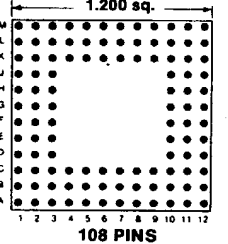
Footprint 12005
