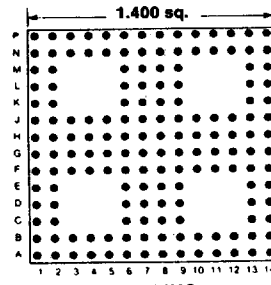
160 PINS Footprint 14009
