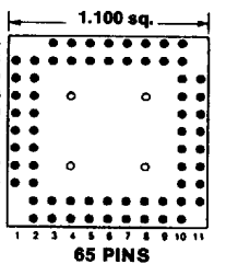
Footprint 11038
