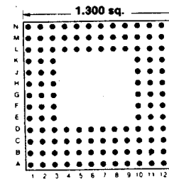
Footprint 13005
