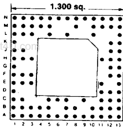
93 PINS Footprint 13045
