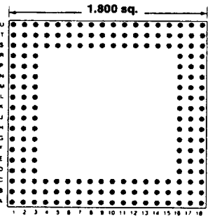
Footprint 18007
