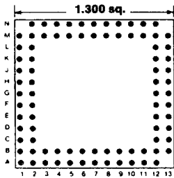
Footprint 13031
