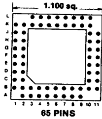
Footprint 11036
