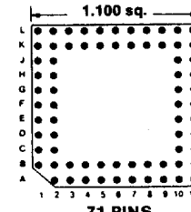
71 PINS Footprint 11027
