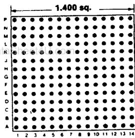
196 PINS Footprint 14001
