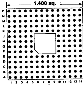
180 PINS Footprint 14002
