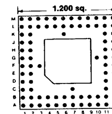
Footprint 12010
