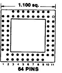
Footprint 11039
