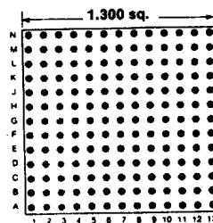
Footprint 13001
