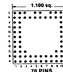
70 PINS
