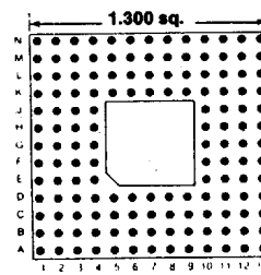
Footprint 13002
