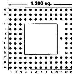
Footprint 13040
