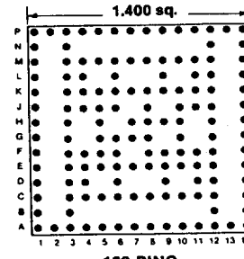
139 PINS Footprint 14010
