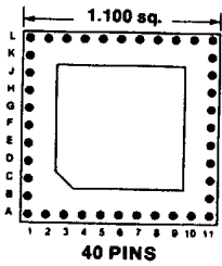
Footprint 11043
