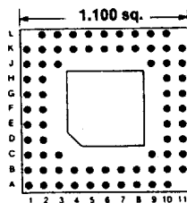
73 PINS Footprint 11021
