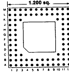
Footprint 12012
