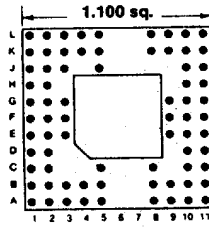
74 PINS Footprint 11017
