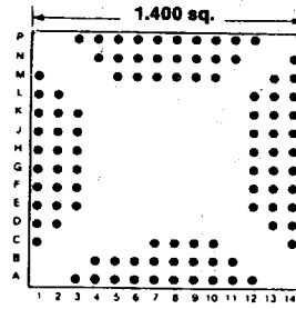
94 PINS Footprint 14022
