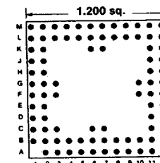
Footprint 12009
