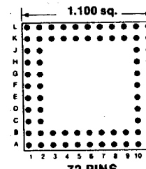
72 PINS Footprint 11024
