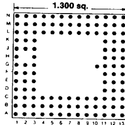
113 PINS Footprint 13050
