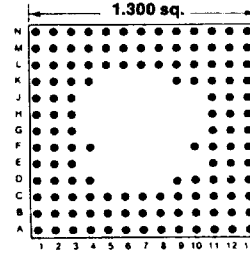
Footprint 13043
