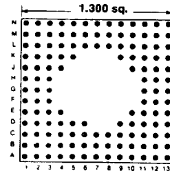
133 PINS Footprint 13055
