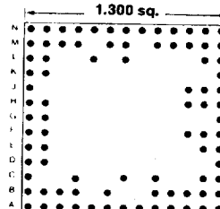
88 PINS Footprint 13057
