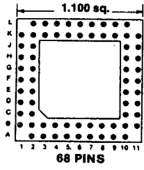
Footprint 11032
