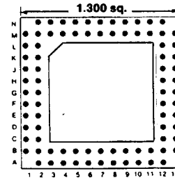
Footprint 13042
