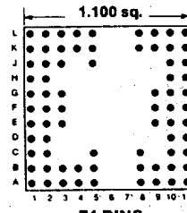
74 PINS Footprint 11018
