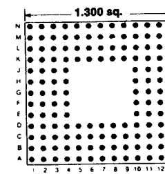
Footprint 13003
