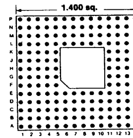
171 PINS Footprint 14007
