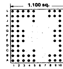
73 PINS Footprint 11020
