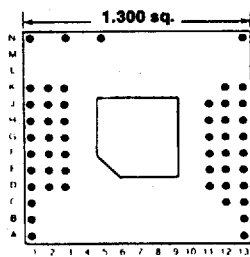
Footprint 13036
