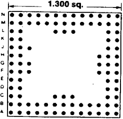
100 PINS Footprint 13059
