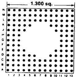
133 PINS Footprint 13046
