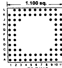
73 PINS Footprint 11022
