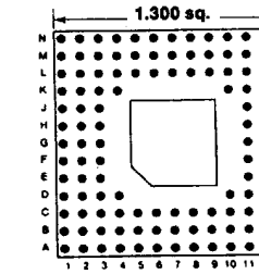
Footprint 13008
