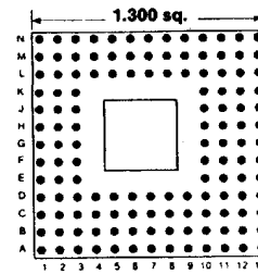
Footprint 13004
