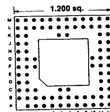
Footprint 12008
