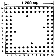
Footprint 12011
