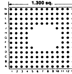
Footprint 13044
