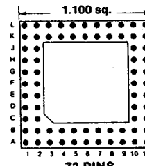
72 PINS Footprint 11023
