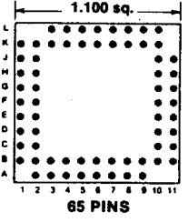
Footprint 11037
