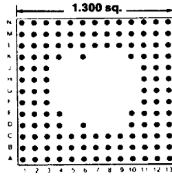
Footprint 13039
