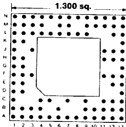
95 PINS Footprint 13047
