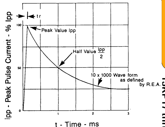
FIGURE 2 Pulse Waveform
