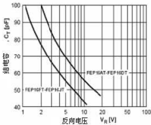
Figure 5. Total Capacitance
