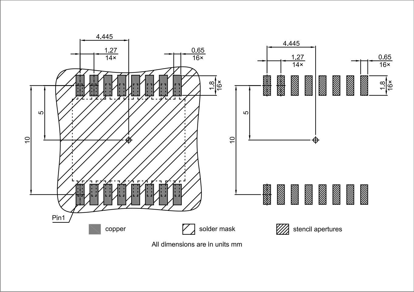
Figure 15 Footprint
