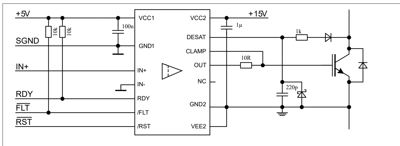
Figure 7 Application example unipolar supply
