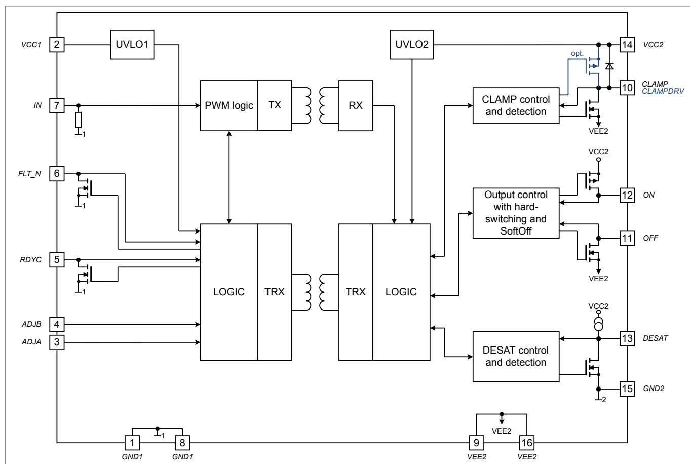
Figure 2 Block diagram
