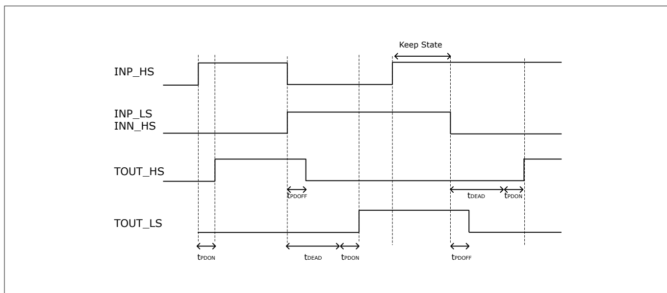
Figure 11 Shoot through protection timing diagram
