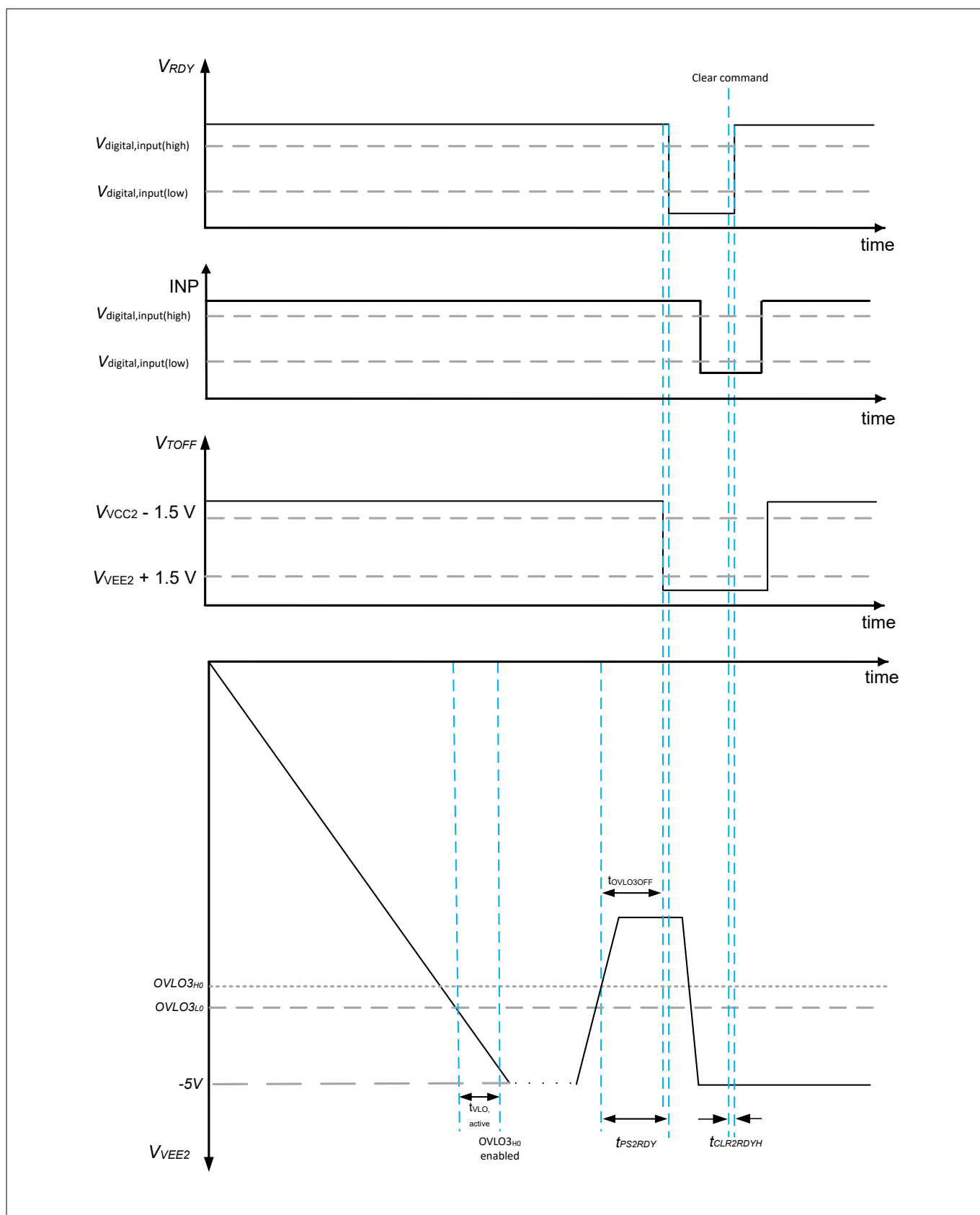
Figure 13 OVLO3 scheme
