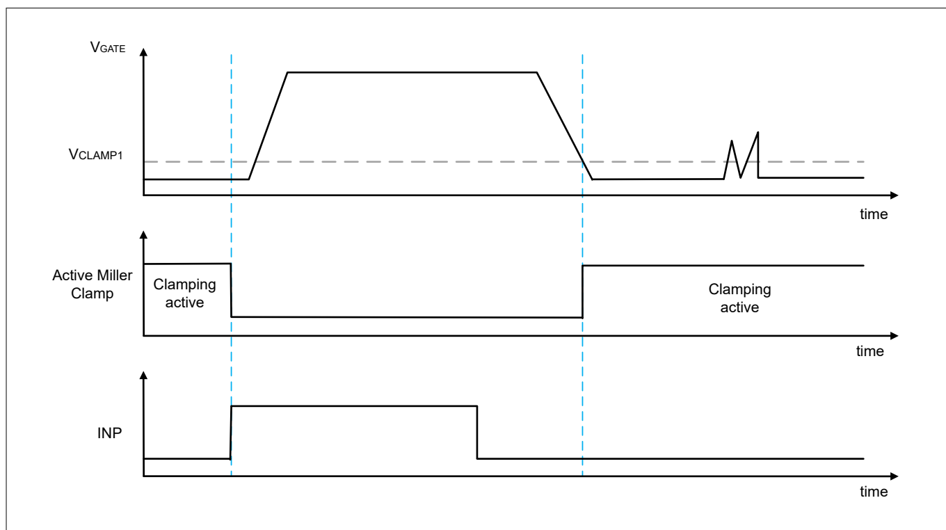
Figure 30 Active Miller clamp timing diagram.
