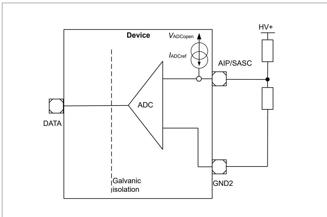
Figure 18 DC-link measurement diagram
