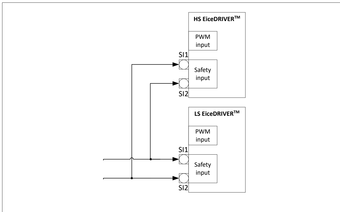
Figure 4 Cross connection of safety inputs in a half bridge configuration
