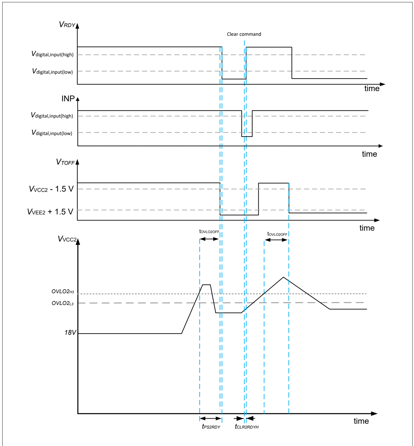
Figure 11 OVLO2 scheme
