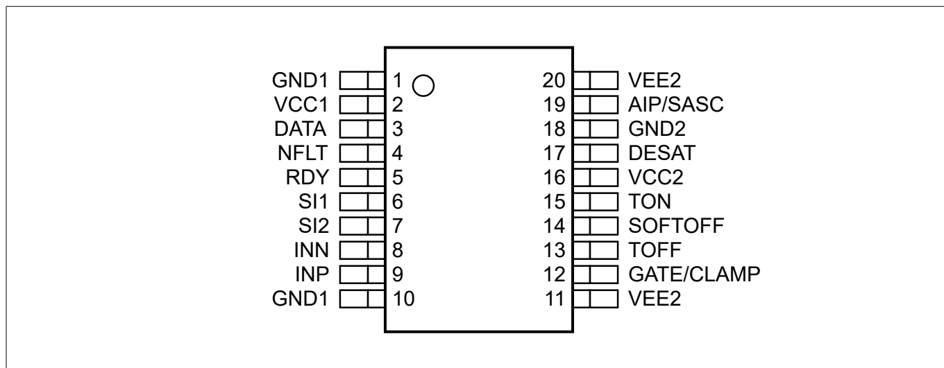
Figure 2 Pin assignment
