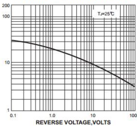
FIG. 5-TYPICAL JUNCTION CAPACITANCE
