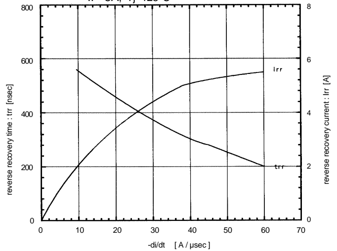
Reverse recovery time characteristics vs. -di/dt IF=5A, Tj=125°C
