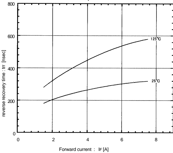
Reverse recovery time vs. Forward current -di/dt=15A / μsec
