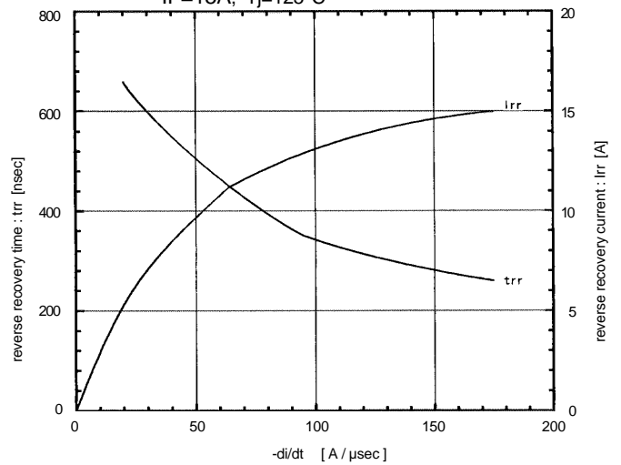
Reverse recovery time characteristics vs. -di/dt IF=15A, Tj=125°C
