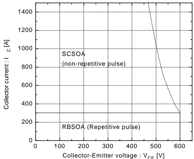
Reversed biased safe operating area +V_{GE}=15V, -V_{GE}\leq 15V, T_J\leq 125^\circ C, R_G\geq 16\Omega
