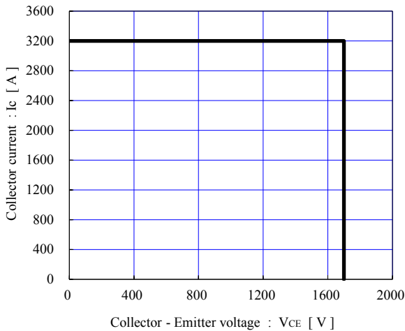
Reverse bias safe operating area (max.) \pm V_{GE}=15V, T_j = 150^\circ C / chip
