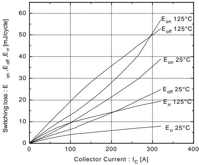
Switching loss vs. Collector current V_{CC}=600V, R_G=4.7\Omega, V_{GE}=\pm 15V
