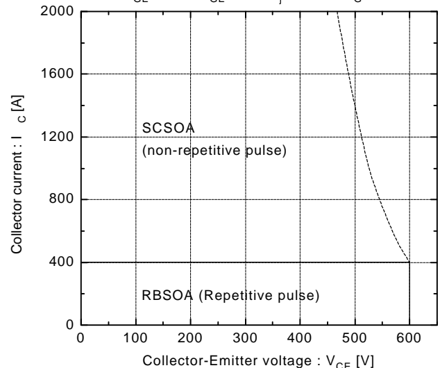
Reversed biased safe operating area +V_{GE}=15V, -V_{GE}\leq 15V, T_J\leq 125^\circ C, R_G\geq 9.1\Omega
