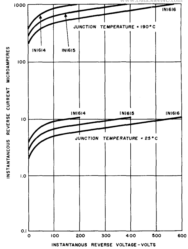
2. REVERSE CHARACTERISTICS
