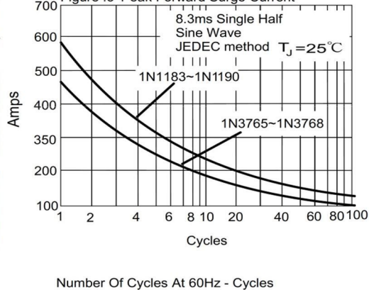
Figure .3- Peak Forward Surge Current
