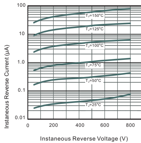
Fig.2 Typical Instaneous Reverse Characteristics
