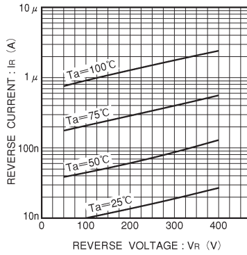
Fig.2 Reverse characteristics
