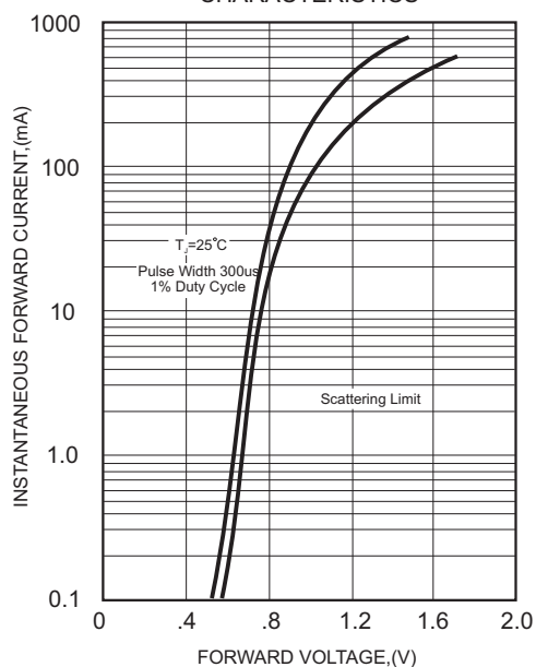
FIG.1-TYPICAL FORWARD CHARACTERISTICS
