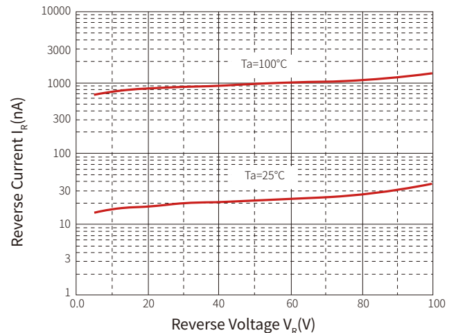
Fig.2 Reverse Characteristics
