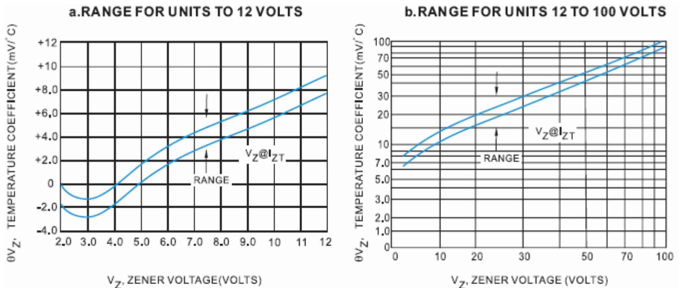
FIG.2 - TEMPERATURE COEFFICIENTS (-55°C to +150°C temperature range;90% of the units are in the ranges indicated.)
