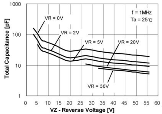
Figure 2. Total Capacitance
