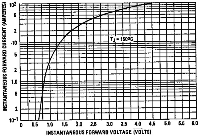
Fig. 3 – Maximum Forward Voltage Vs. Forward Current, 1N4816-22, 1N5052-54, 10D Series
