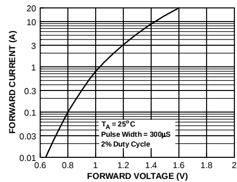
Forward Characteristics
