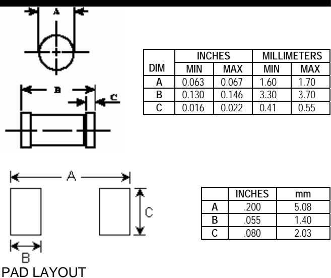
PAD LAYOUT
