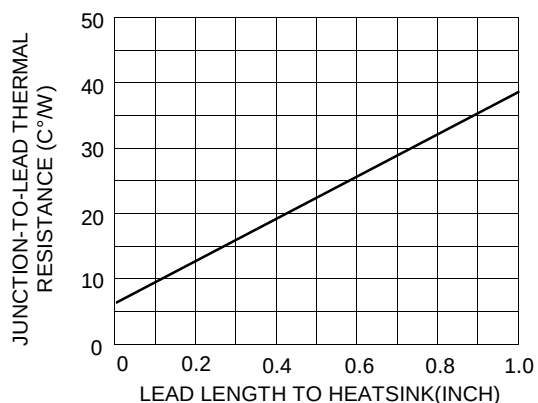
Fig. 2 TYPICAL THERMAL RESISTANCE
