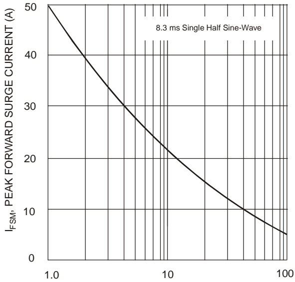
NUMBER OF CYCLES AT 60Hz
