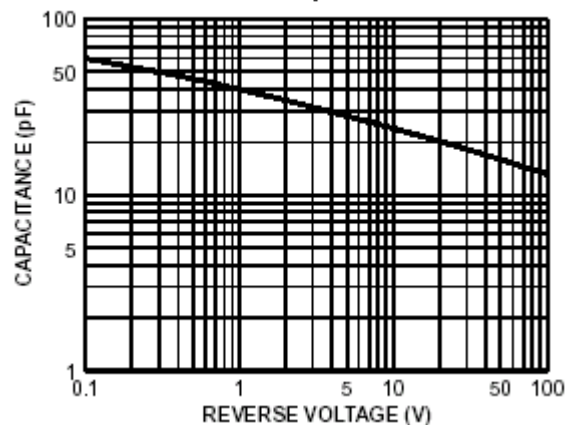
Junction Capacitance
