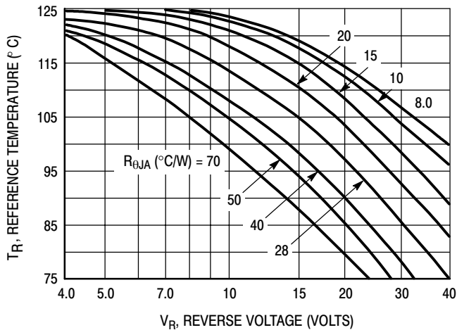
Figure 3. Maximum Reference Temperature 1N5825
