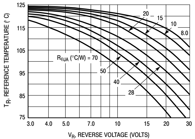
Figure 2. Maximum Reference Temperature 1N5824
