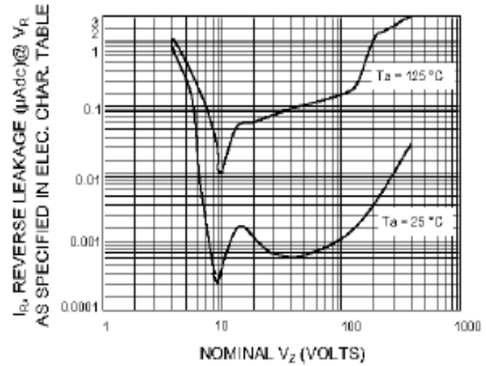
TYPICAL REVERSE LEAKAGE
