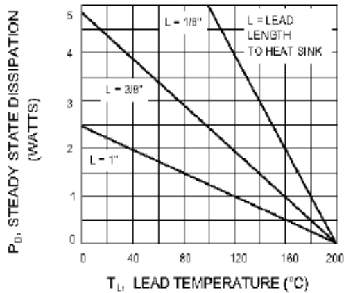
POWER TEMPERATURE DERATING CURVE
