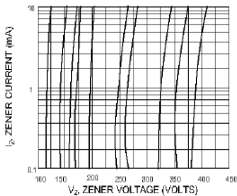
ZENER VOLTAGE VS. ZENER CURRENT V_Z = 100 thru 400 VOLTS
