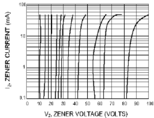
ZENER VOLTAGE VS. ZENER CURRENT V_Z = 12 thru 82 VOLTS
