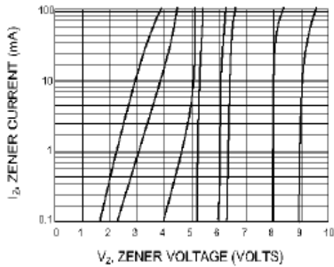
ZENER VOLTAGE VS. ZENER CURRENT V_Z = 3.3 thru 10 VOLTS
