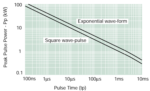
Figure 3 - Peak Pulse Power vs. Pulse Time
