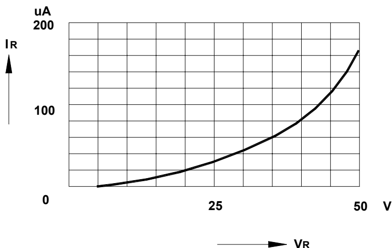
Reverse Characteristics
