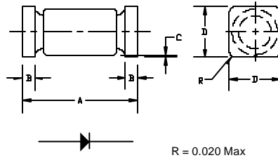
500 W 1N6102US - 1N6137US, 1N6102AUS - 1N6137AUS
