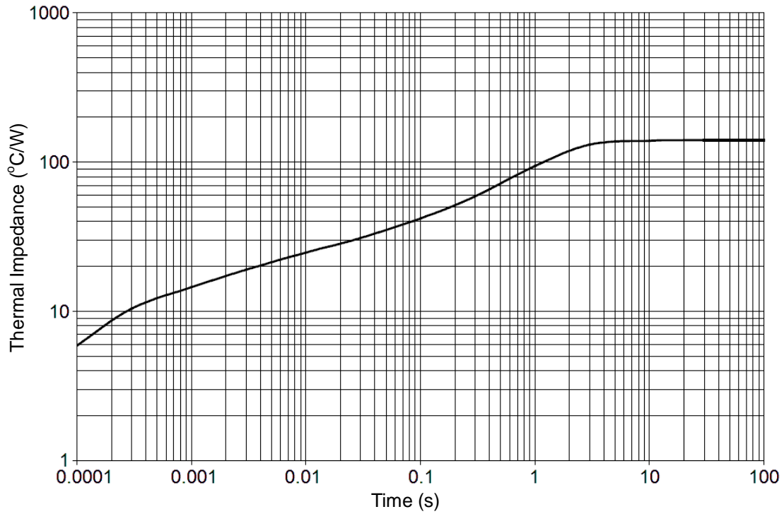
FIGURE 3 Maximum Thermal Impedance at T_L = 25^\circ\text{C}
