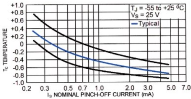
Temperature Coefficient
