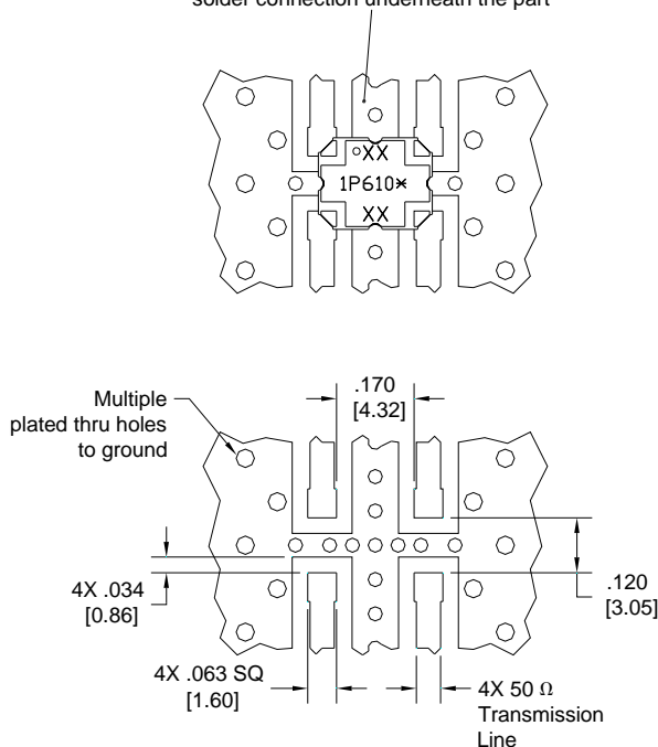
Dimensions are in Inches [Millimeters] 1P610* Rev A Mounting Footprint
