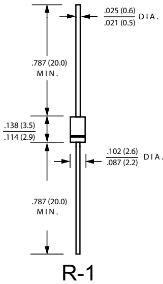
R-1 Dimensions in inches and (millimeters)
