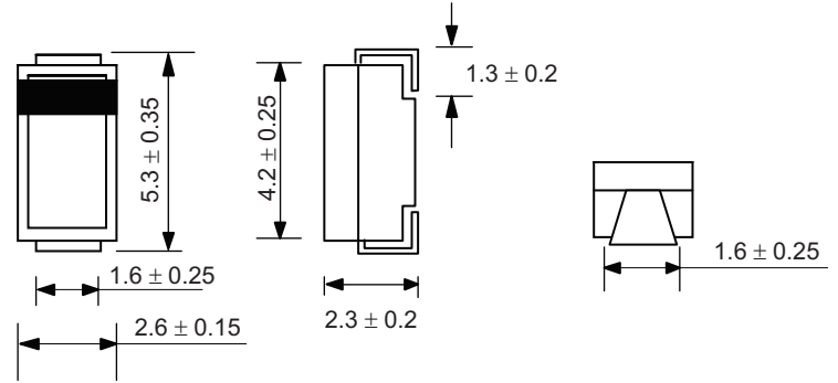
SMA Dimensions in millimeters
