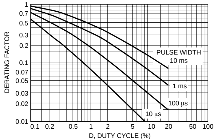
Figure 6. Typical Derating Factor for Duty Cycle
