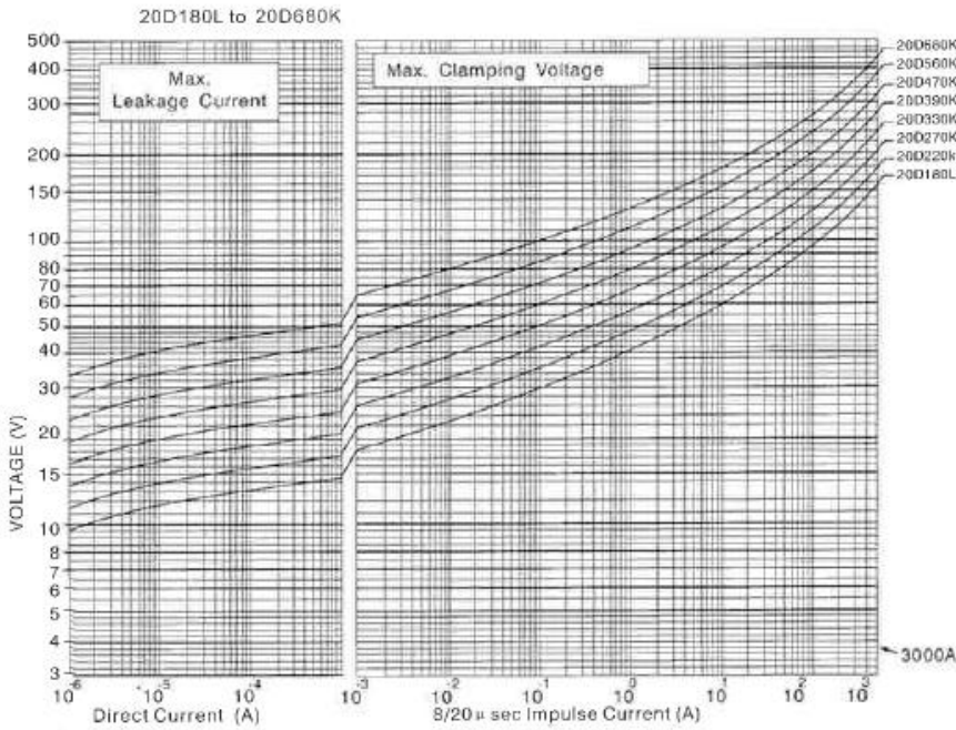
V-I curve
