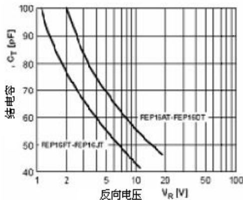
Figure 5. Total Capacitance
